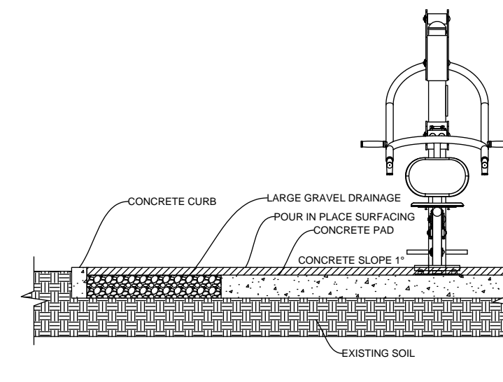
French Drain #2
