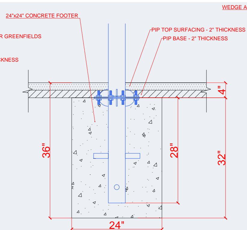
PIP SURFACING
