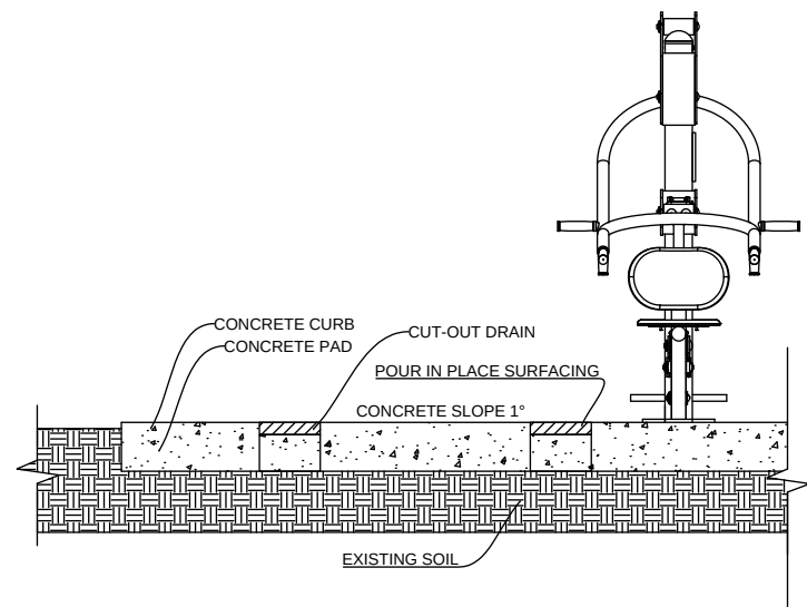
Curb Cutouts
