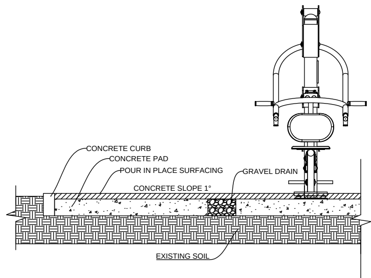
French Drain #1
